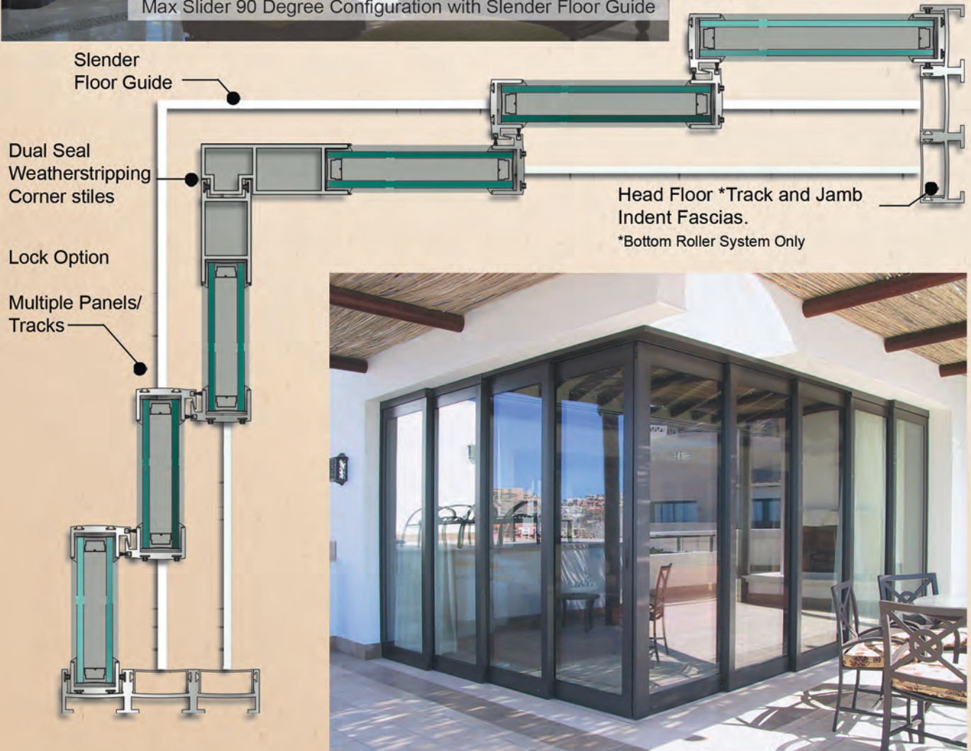
Max Slider 90 Degree Configuration with Slender Floor Guide
