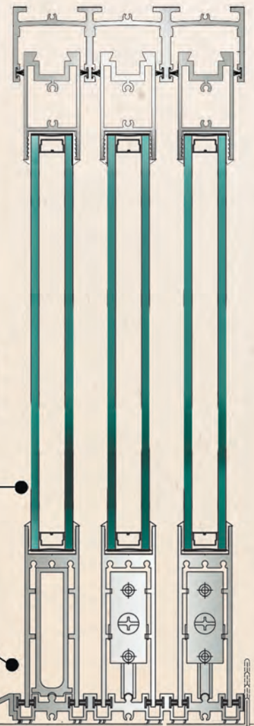
Max Multi Track In-Line Sliding System
