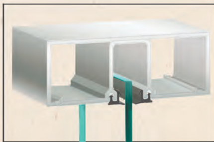
1 3/4" H X 4 1/2" W PL-450SH
