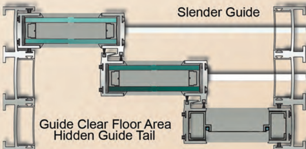
Max Slider with Slender Floor Guide
