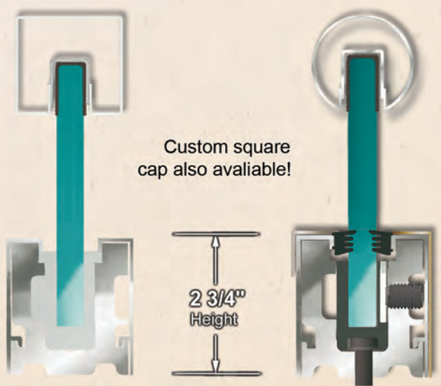
PL- DSMHRB 2 1/2" w x 2 3/4" h
