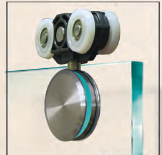
PL-RSCBS ROUND SLIDING ROLLER 2 3/8" DIA
