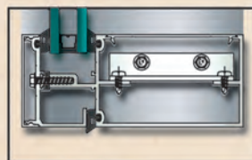
SILL
