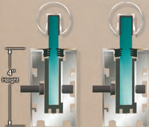
PL- DSHRB / PL-TC 2 1/2" w x 4" h
